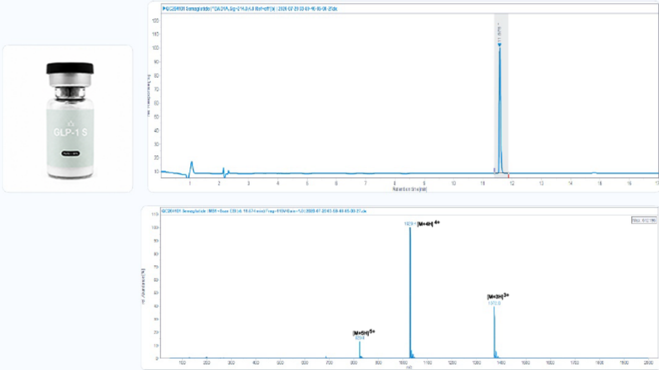
HPLC Chromatogram (Retention Time: 11.576 min)
